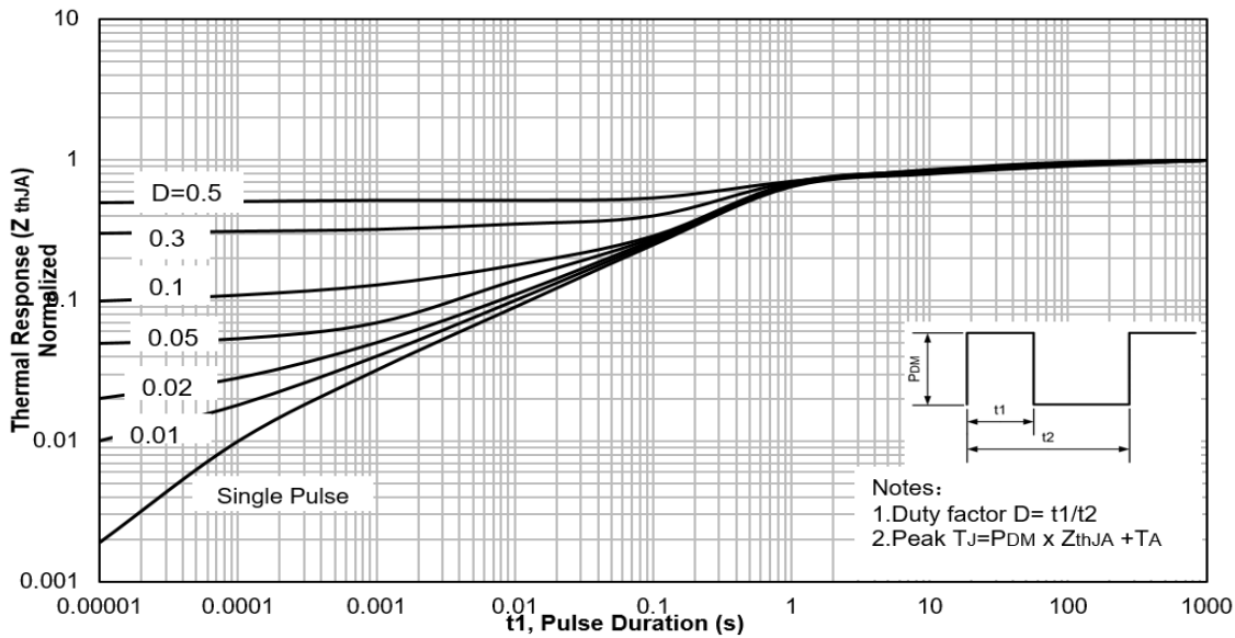
Figure 9. Maximum Effective Transient Thermal Impedance ,Junction-to-Ambient
