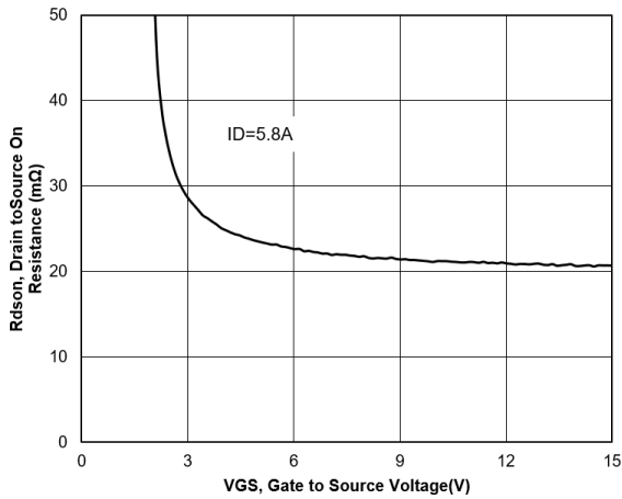
Figure 7. Typical Drain to Source ON Resistance
