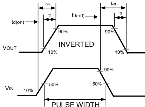
Figure 10. Switching wave
